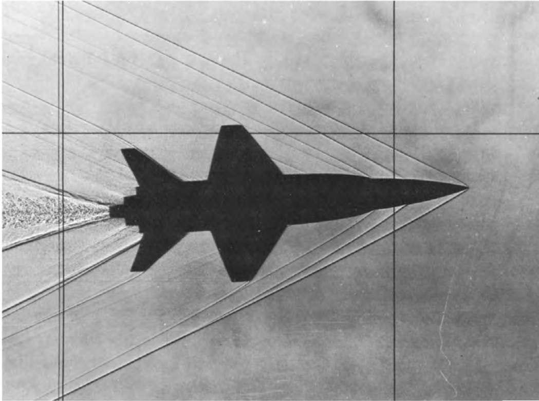
These dramatic photographs of free-flight models of the X-15 being fired into a wind tunnel vividly detail the shock-wave patterns for airflow at Mach 3.5 (above) and at Mach 6.
