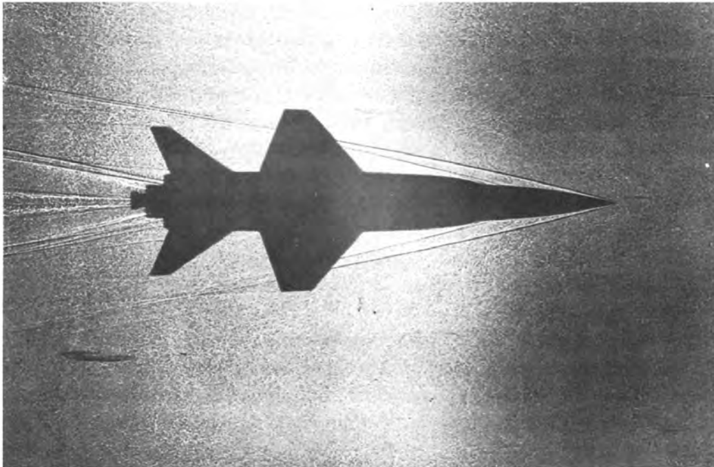
These dramatic photographs of free-flight models of the X-15 being fired into a wind tunnel vividly detail the shock-wave patterns for airflow at Mach 3.5 (above) and at Mach 6.
