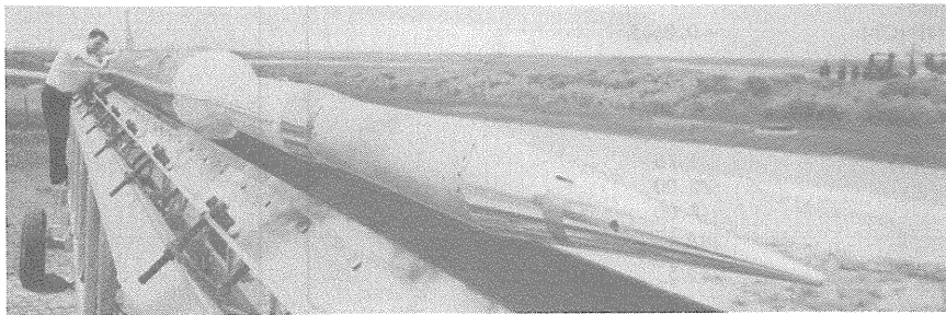
Figure 32a - Aerobee 300A, side view.
