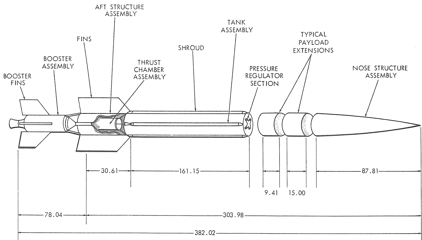
(b) Outline drawing.
