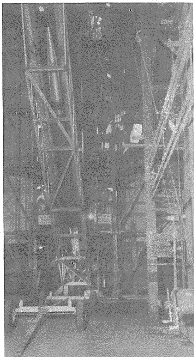
(h) Lifting of launch rail dolly and sounding rocket into launch tower.
