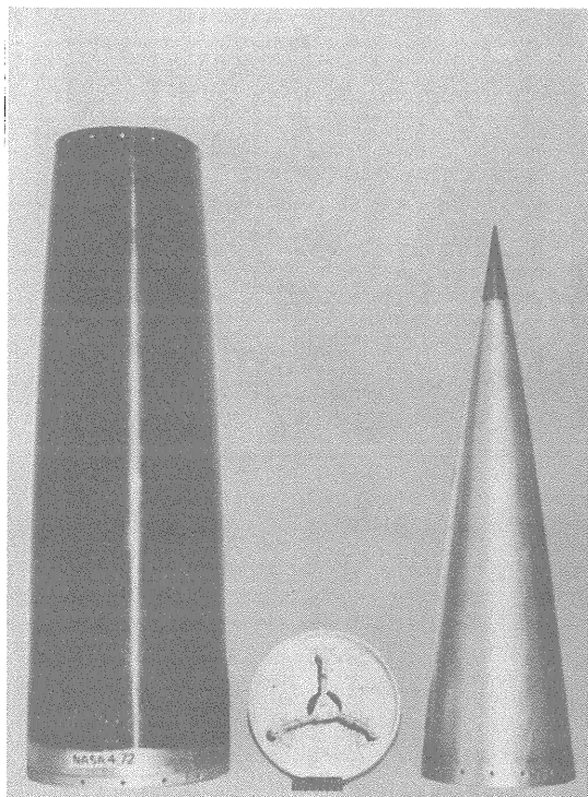
(a) Ogive nose cone and ejection mechanism showing aft side of release cam bulkhead.
