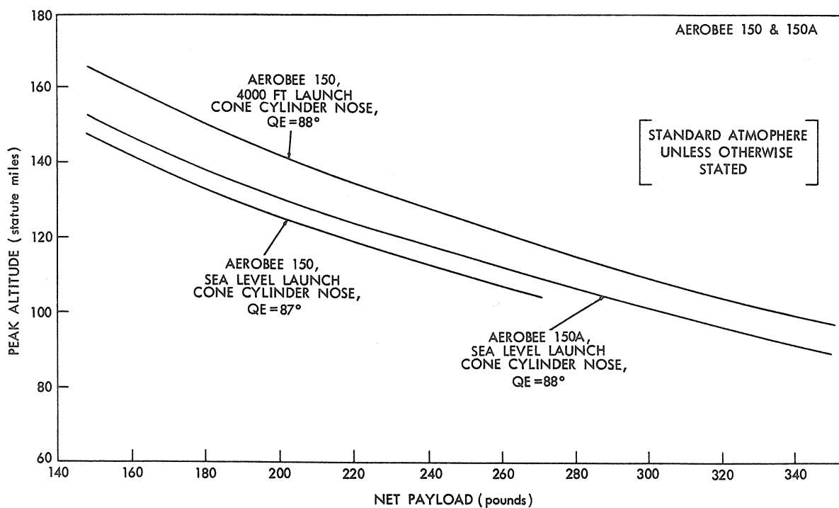
Figure A2 - Peak altitude versus net payload for cone-cylinder nose cones.
