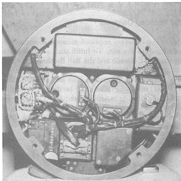
(c) Top view showing location of parts, routing of plumbing, and orientation between ACS and forward skirt.
