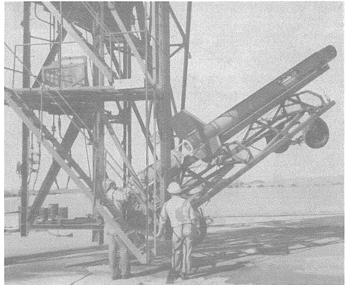
(h) Sounding rocket being lifted into launch tower.
