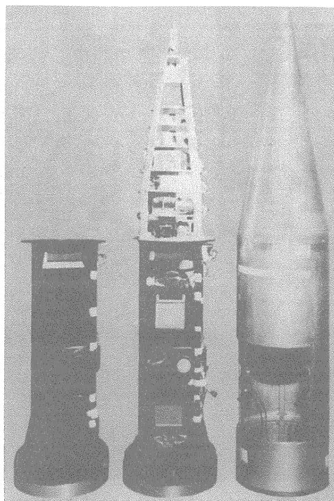
(b) Typical instrumentation package with cone-cylinder nose cone.
