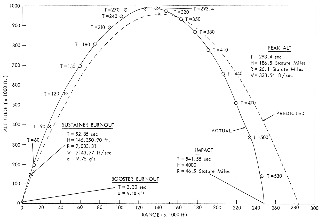
Figure 20 - Flight 4.30 GG - altitude vs. range.
