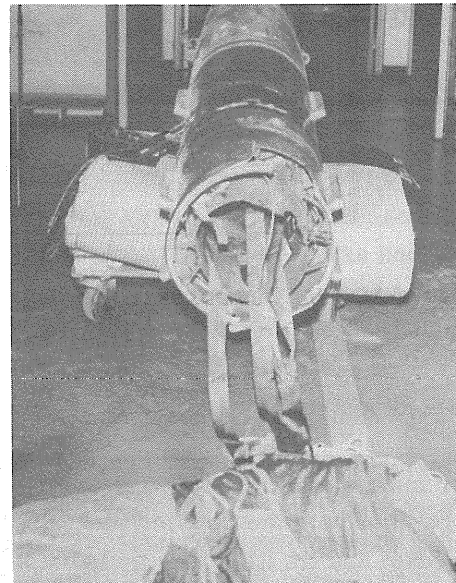
(b) Payload after recovery showing parachute attachments.
