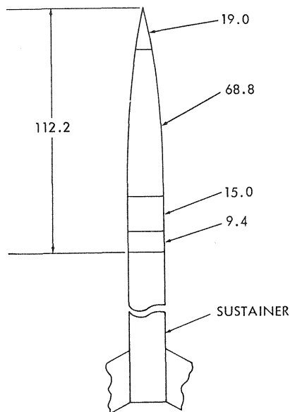
Figure 27 - Flight 4.09 GA - payload dimensions and flight characteristics.
