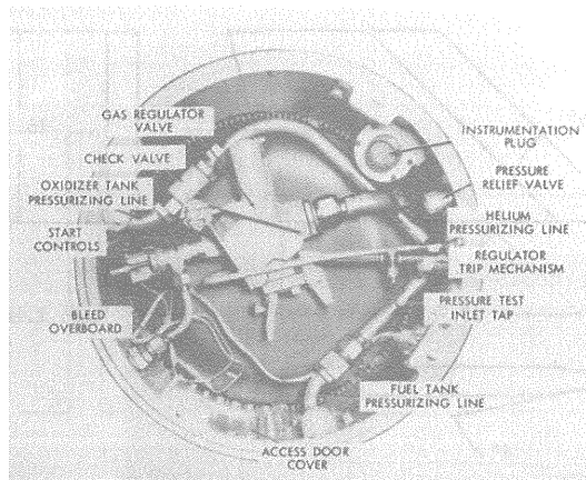
Figure 12 - Aerobee 150 forward skirt, showing locations of pressurizing system components.
