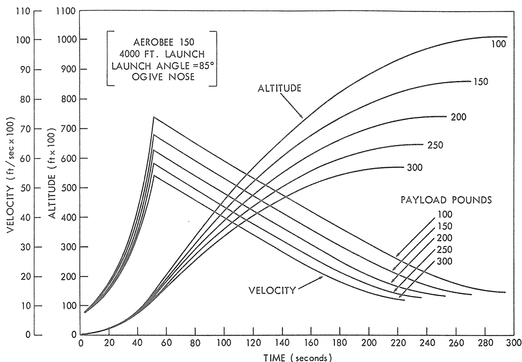
Figure B - Aerobee 150 Velocity and Altitude Versus Time for Various Payload Weights.
