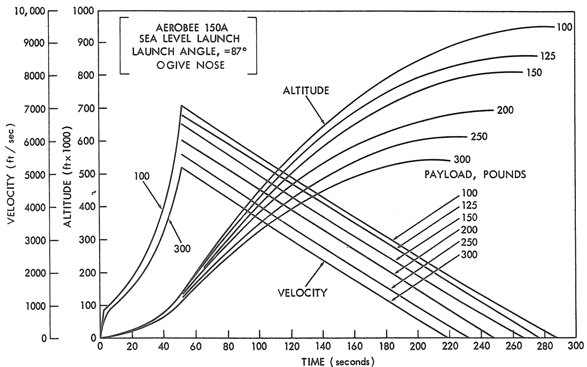
Figure A4 - Aerobee 150A velocity and altitude versus time for various payloads.
