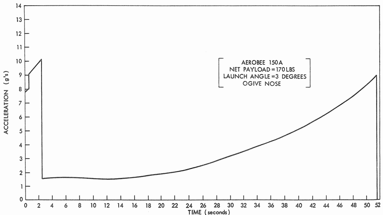
Figure A6 - Acceleration versus time for Aerobee 150A (typical).
