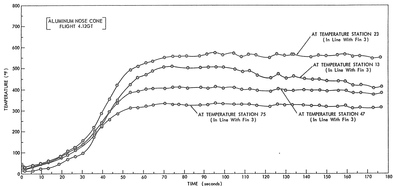
Figure B1 - Representative flight temperatures for ogival nose cones.
