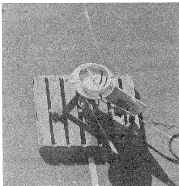
(g) Ground test of three-wrap yo-yo despin system.
