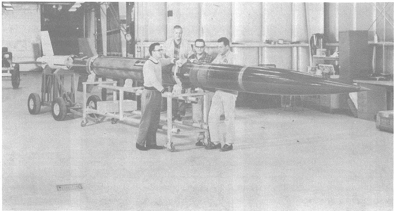
(a) Photo of assembled rocket, payload, and booster motor.
