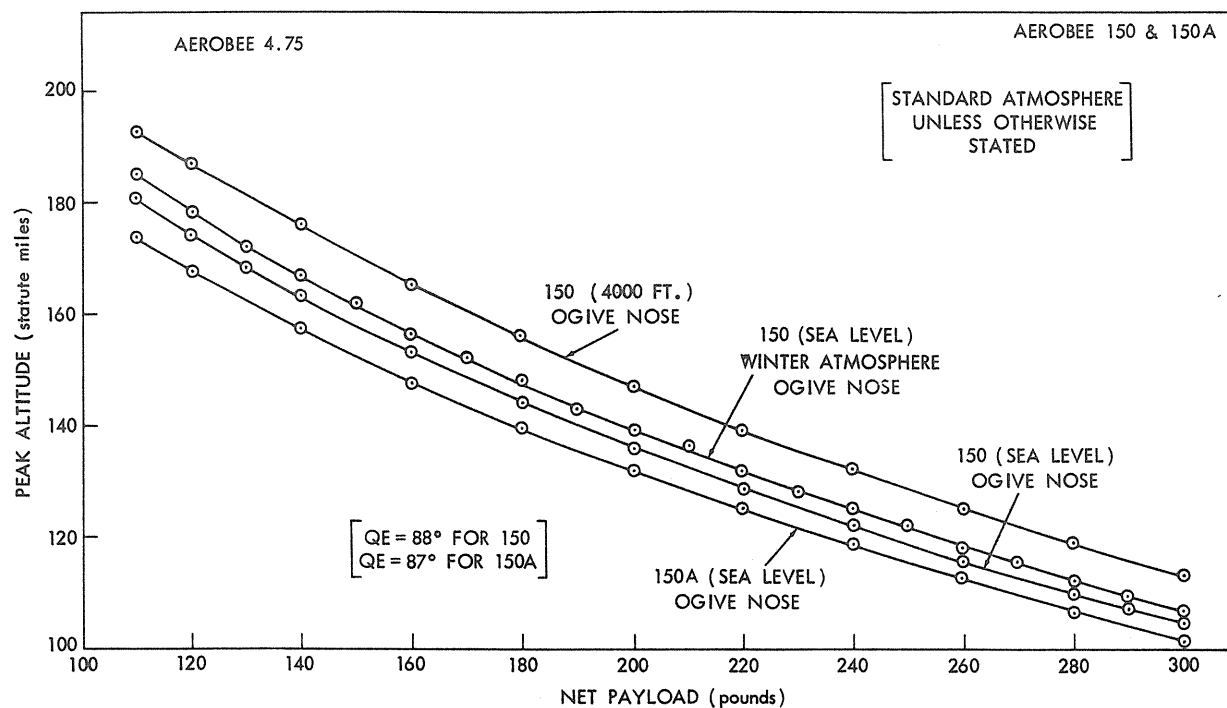
Figure A1 - Peak altitude versus net payload for ogival nose cones.
