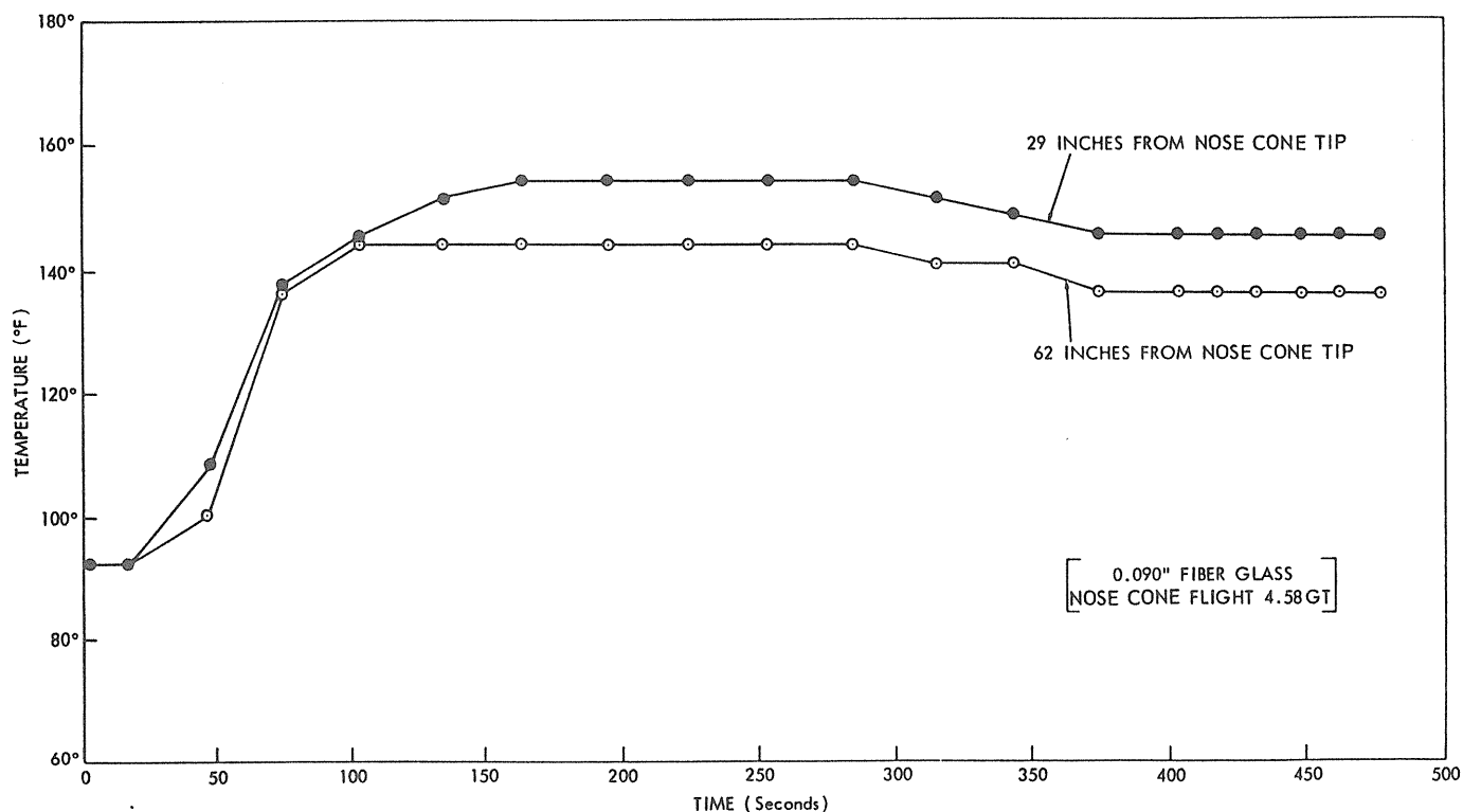
Figure B2 - Representative flight temperatures for ogival nose cones.
