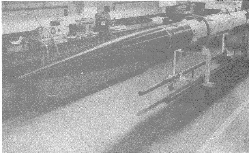
Figure 31 - Aerobee 100 (Junior) on assembly dolly.
