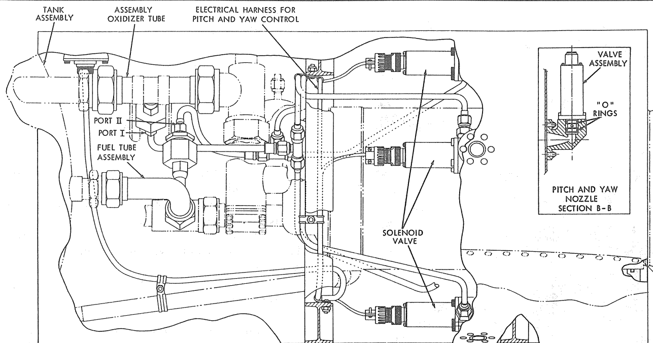
(a) Cutaway drawing showing electrical and mechanical installation of ACS pitch and yaw jets in the tail can. (b) Side view of pitch/yaw nozzle.
