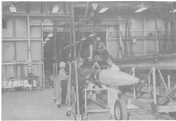
(e) Transfer of sounding rocket from assembly dolly to launch rail dolly, Step 1.
