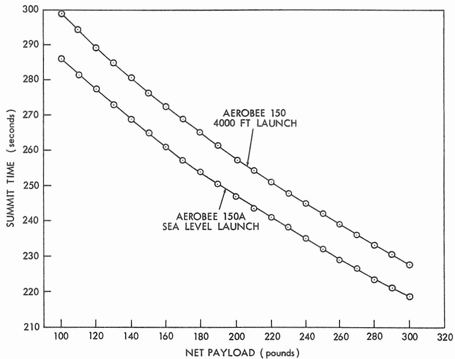
Figure A5 - Summit time versus net payload for Aerobee 150 and 150A sounding rockets with ogival nose cones and a QE = 87°.
