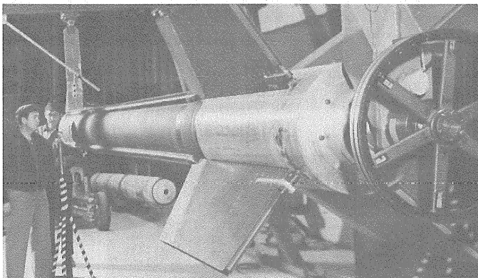
(a) Sustainer motor on horizontal spin unit.
