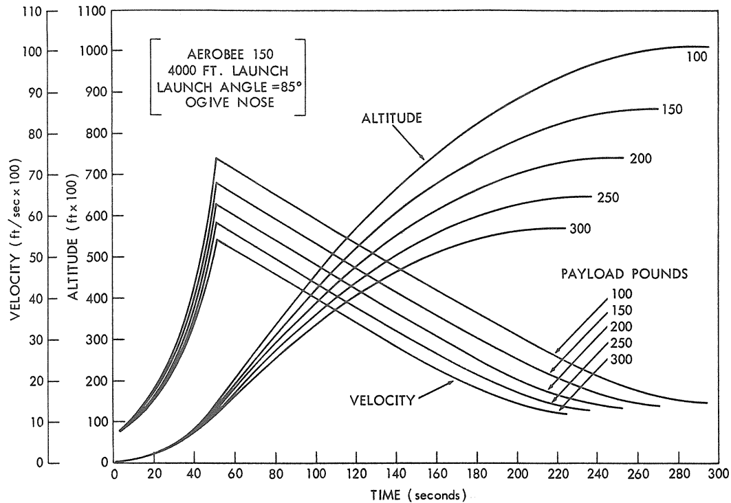
Figure A3 - Aerobee 150 velocity and altitude versus time for various payloads.
