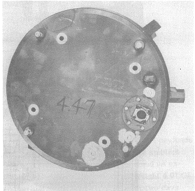
(a) Top view of parachute extension bulkhead.
