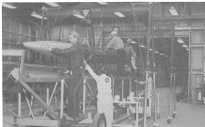
(f) Transfer of sounding rocket from assembly dolly to launch rail dolly, Step 2.
