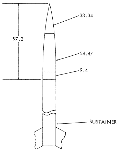
Figure 21 - Flight 4.30 GG - payload dimensions and flight characteristics.
