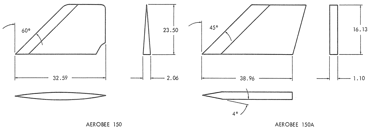
Figure 10 - Aerobee tail fin configuration.
