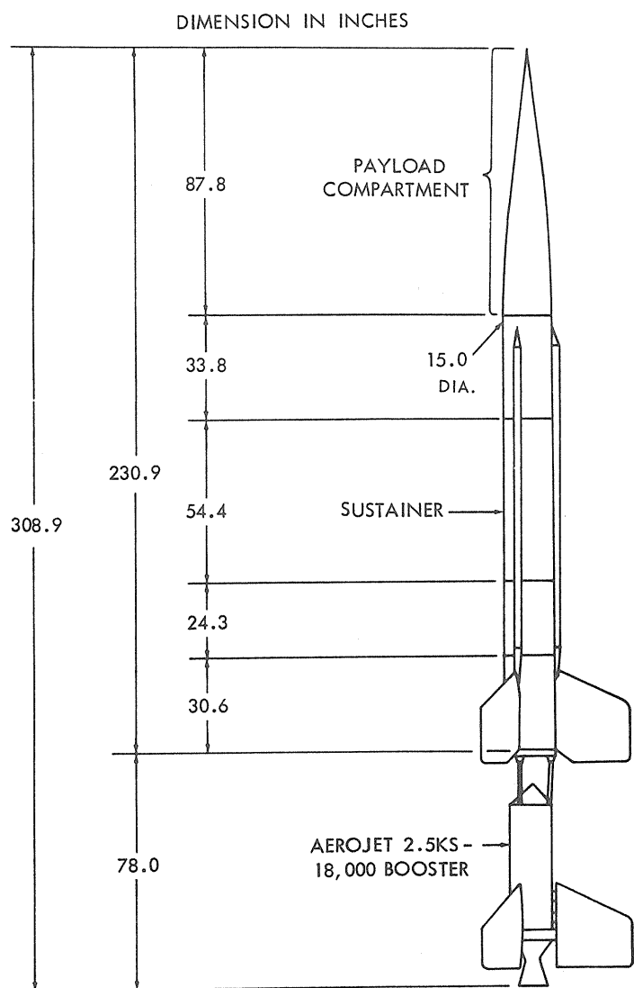
Figure 17 - Aerobee 100 outline drawing.
