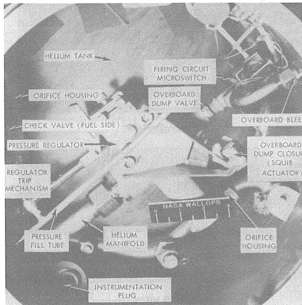
(a) Forward skirt.
